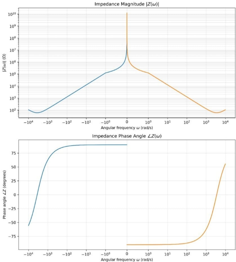
Fig. 21.1. Impedance mag vs angular frequency, Impedance phase angle vs angular frequency
