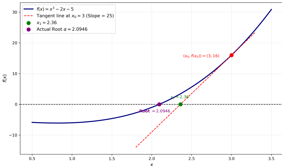
Fig. 22.1. Newton Raphson iteration for f(x)
