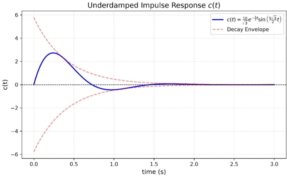
Fig. 6.1. c(t) vs time
