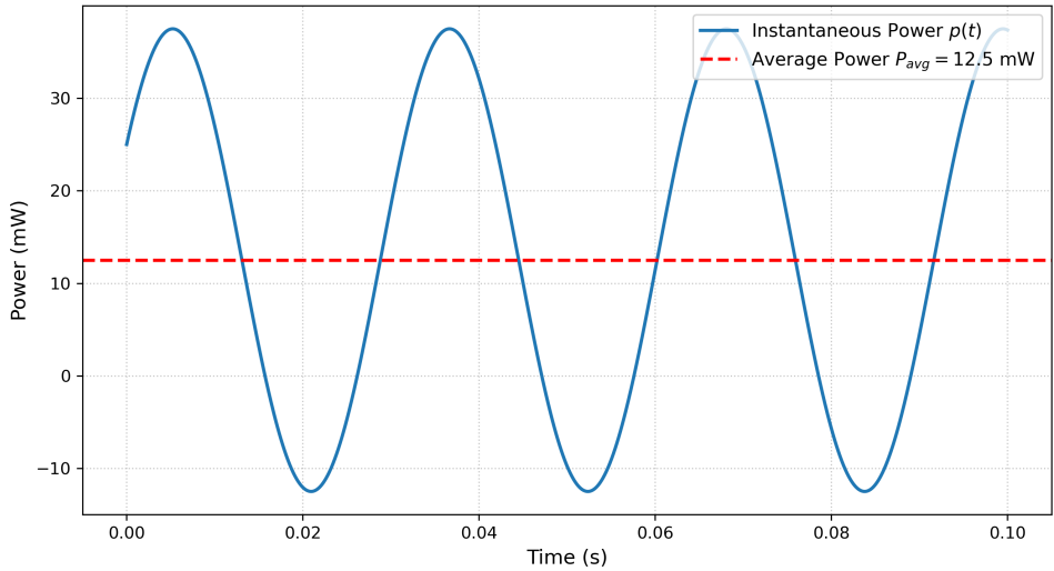
Fig. 11.1. Power vs time
