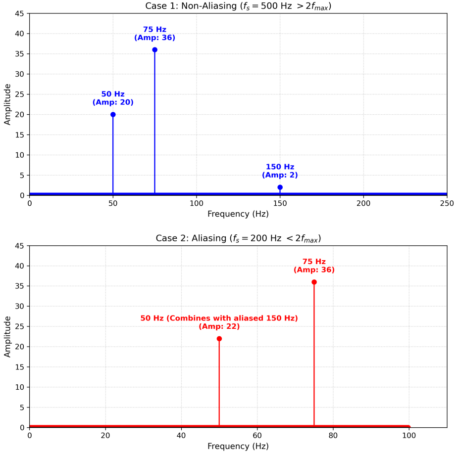
Fig. 10.1. Aliasing and Non-Aliasing
