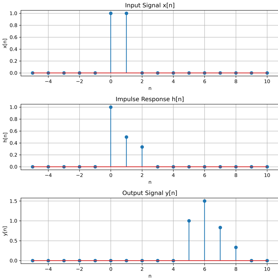
Fig. 17.1. x[n], h[n], y[n] vs n
