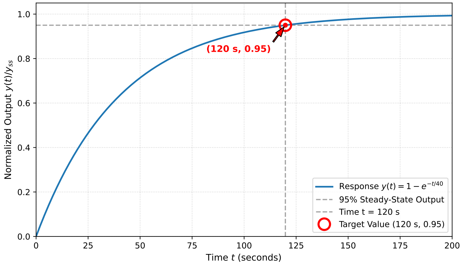
First-Order System Step Response ( \tau = 40 s)
