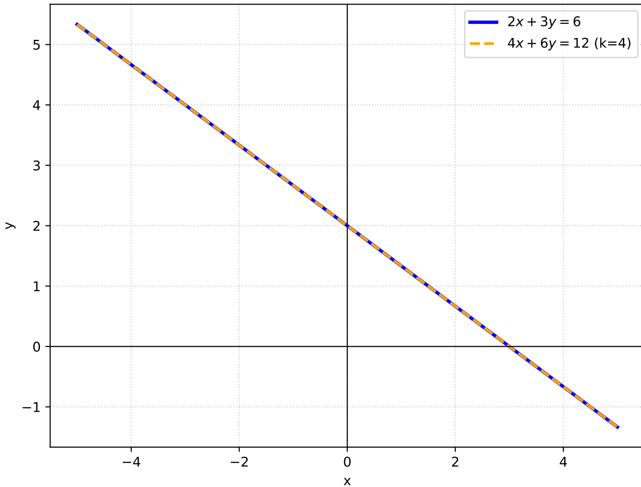
k = 4: Lines Overlap (Coincident - Infinitely Many Solutions)
