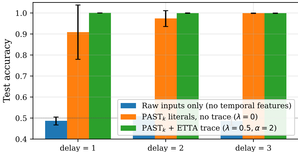
Temporal-XOR: temporal literals + ETТА trace each contribut
