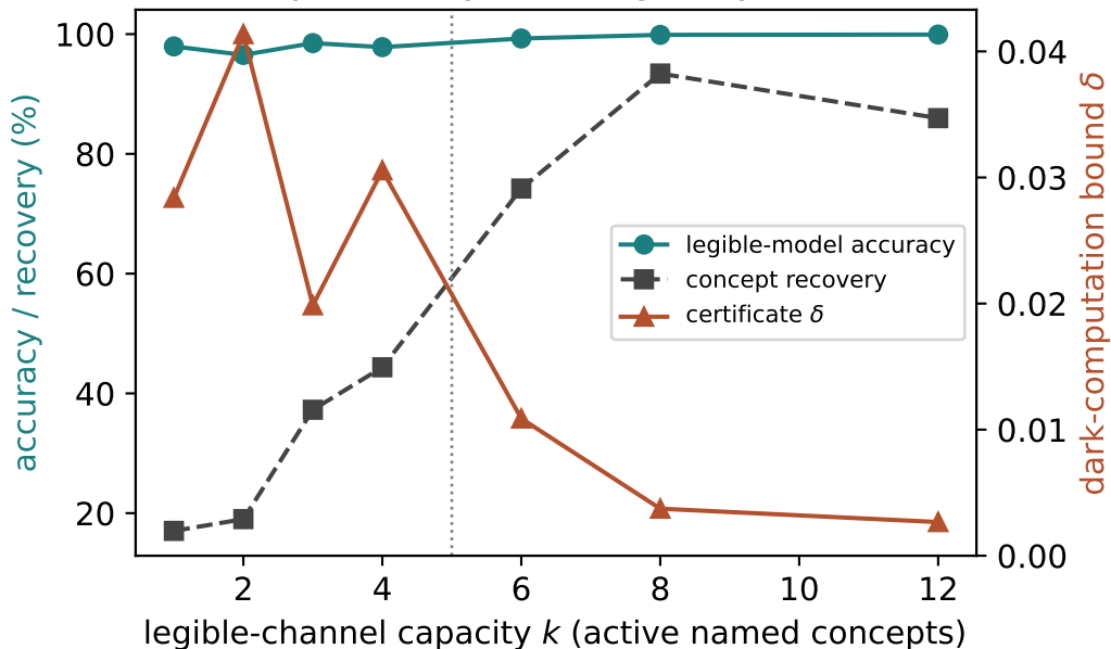
Interpretability-tax / legibility frontier
