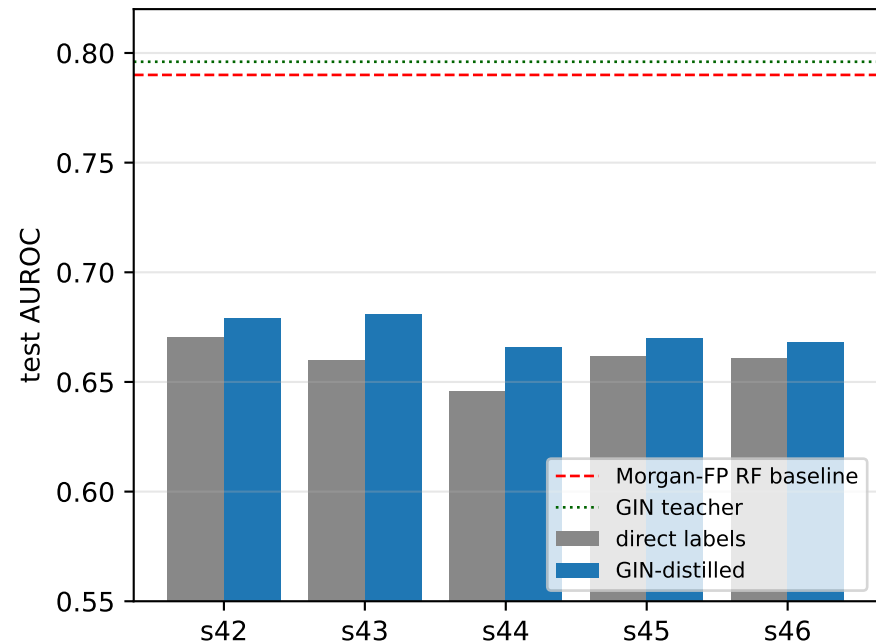
Per-seed test AUROC (TDC AMES)
