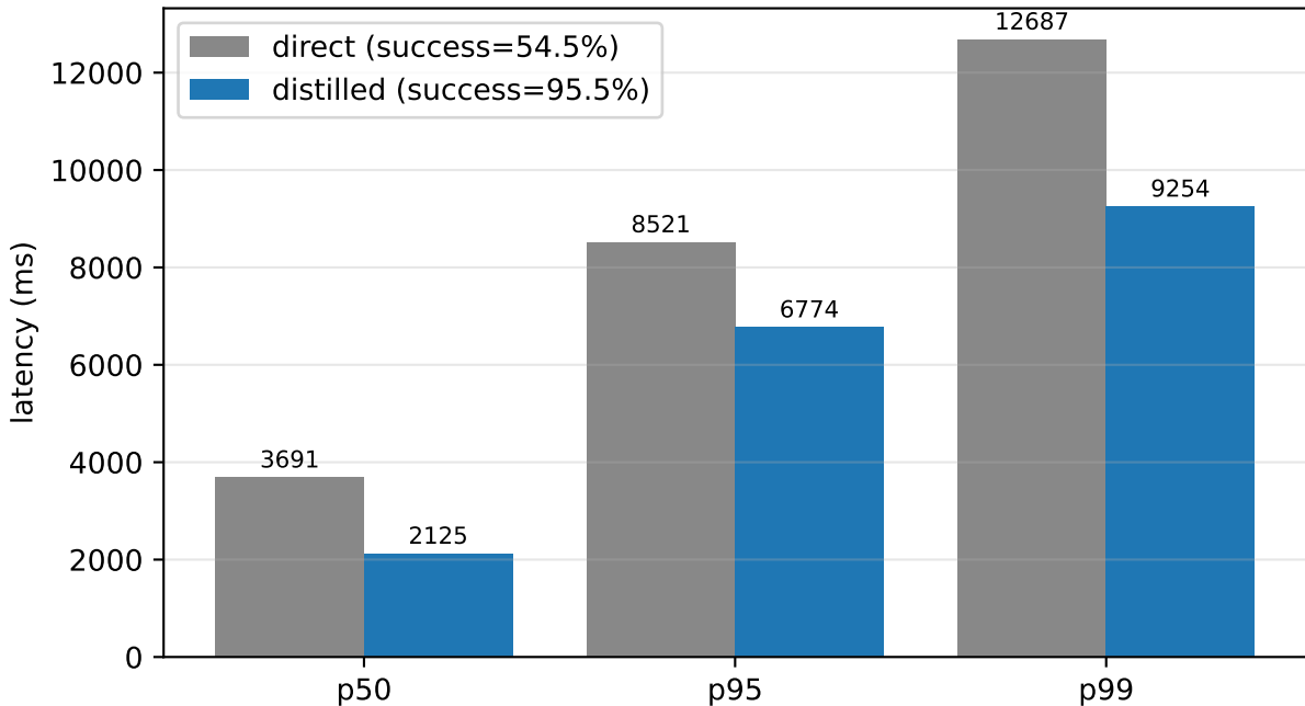
Counterfactual recourse latency on TDC AMES (per molecule, ensemble-of-5)
