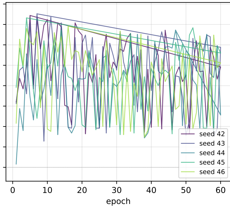
Phase 2: GIN-distilled
