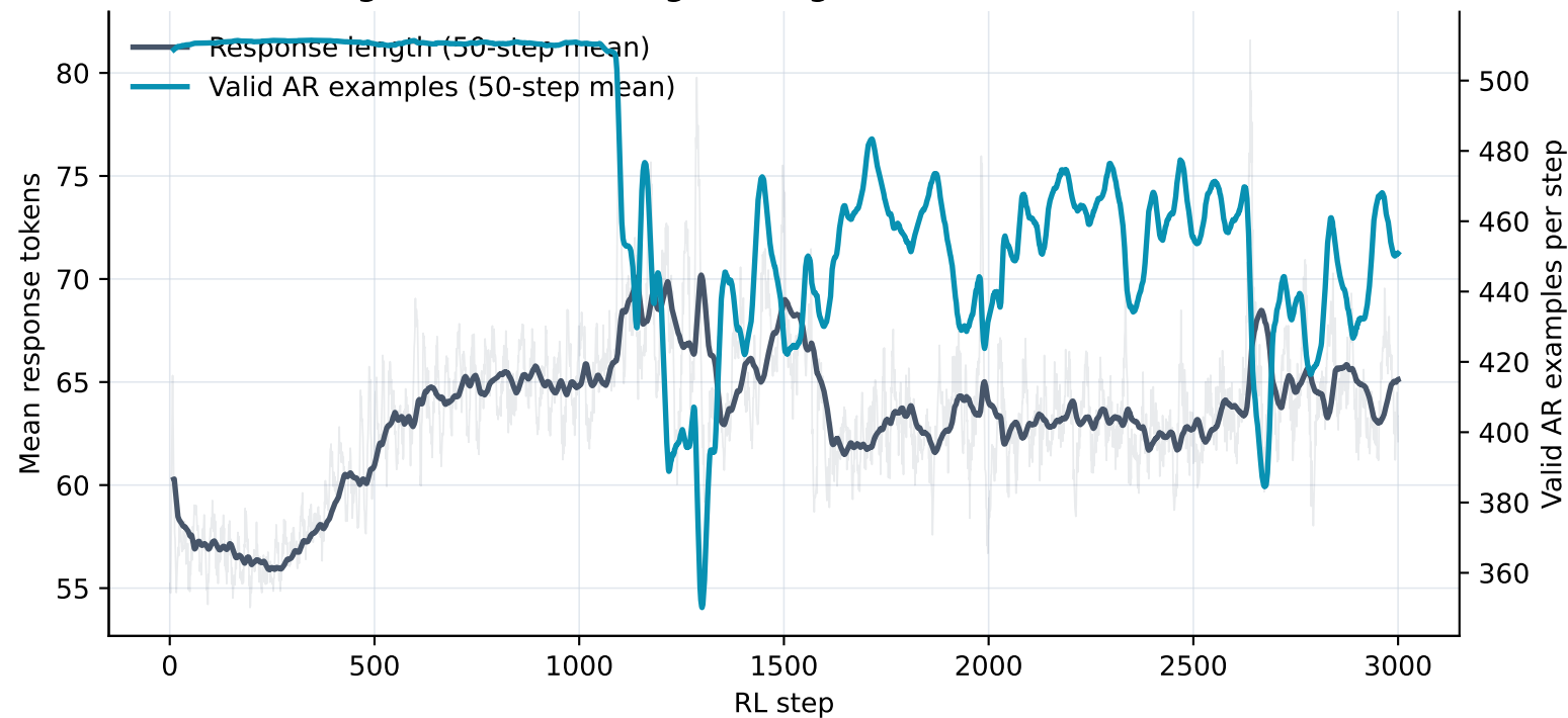
Generation length and AR training coverage
