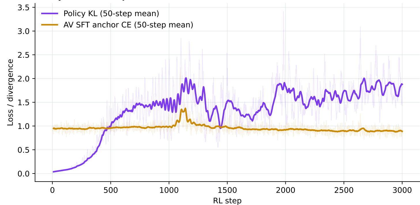
Policy drift and supervised anchor
