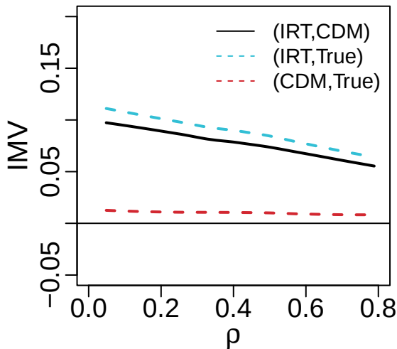
DINA with MP
