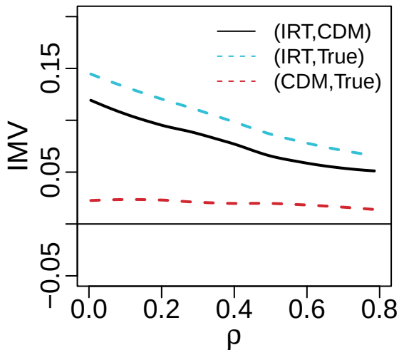
G-DINA with MP
