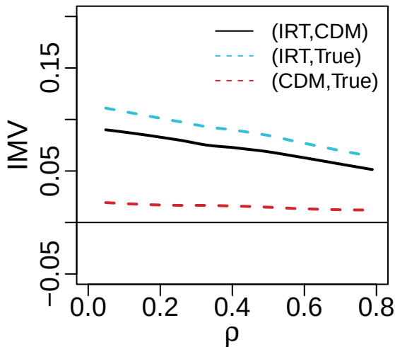
DINA with MAP
