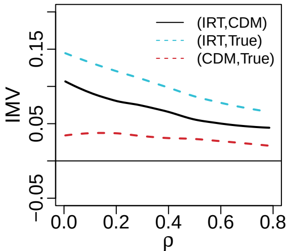
G-DINA with MAP
