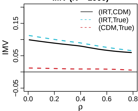
IMV (N = 1000)
