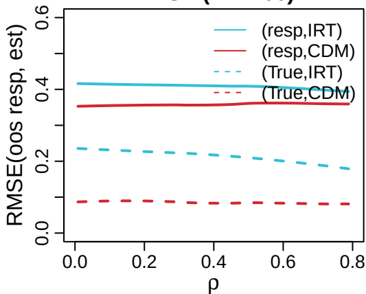
RMSE (N = 200)
