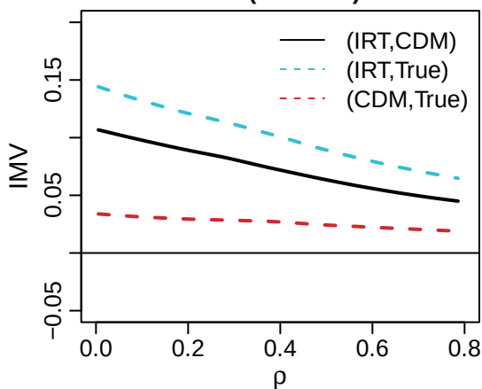
IMV (N = 1000)
