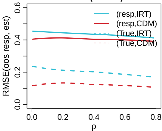
RMSE (N = 200)
