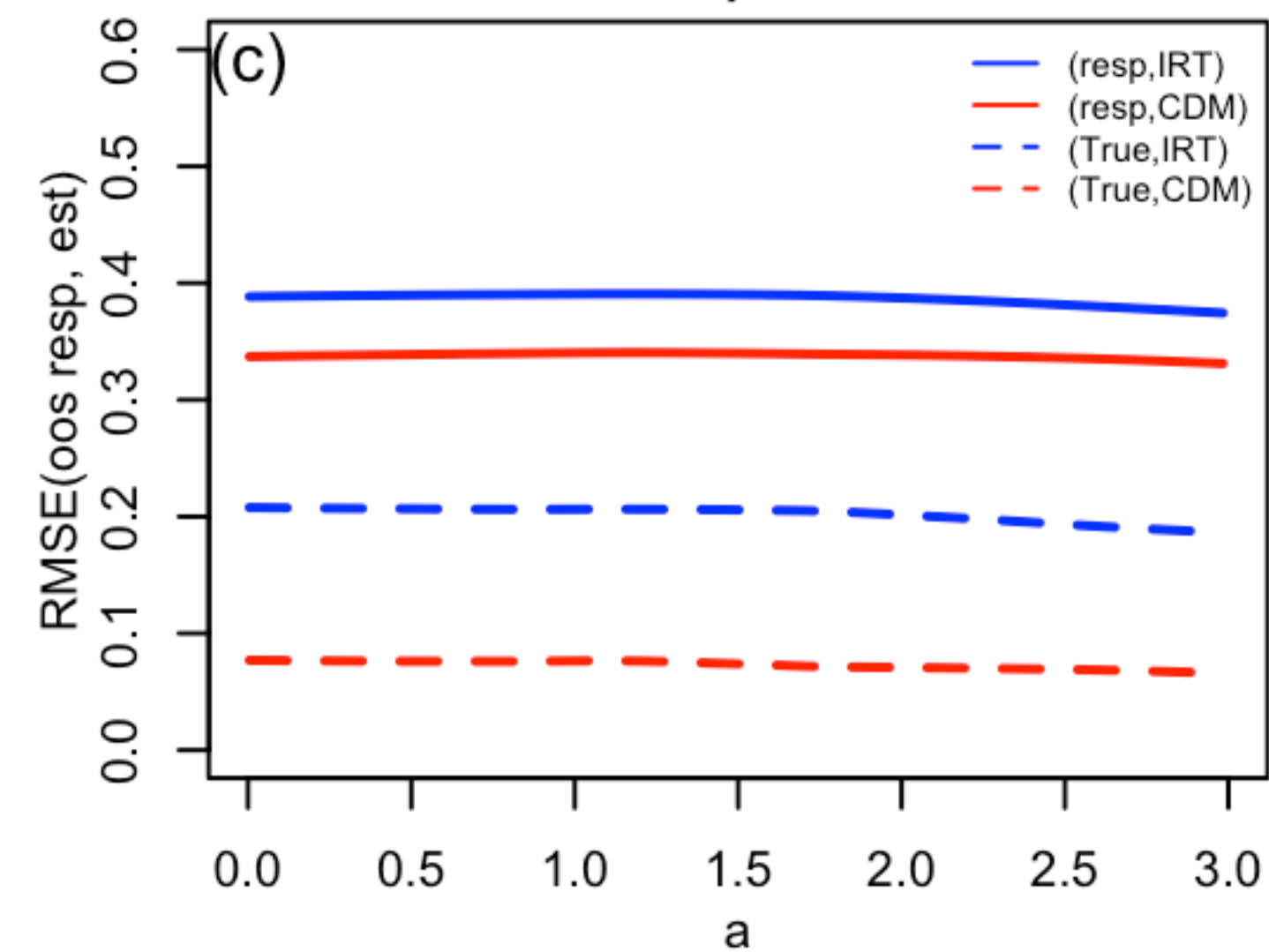
RMSE ps = 0.4
