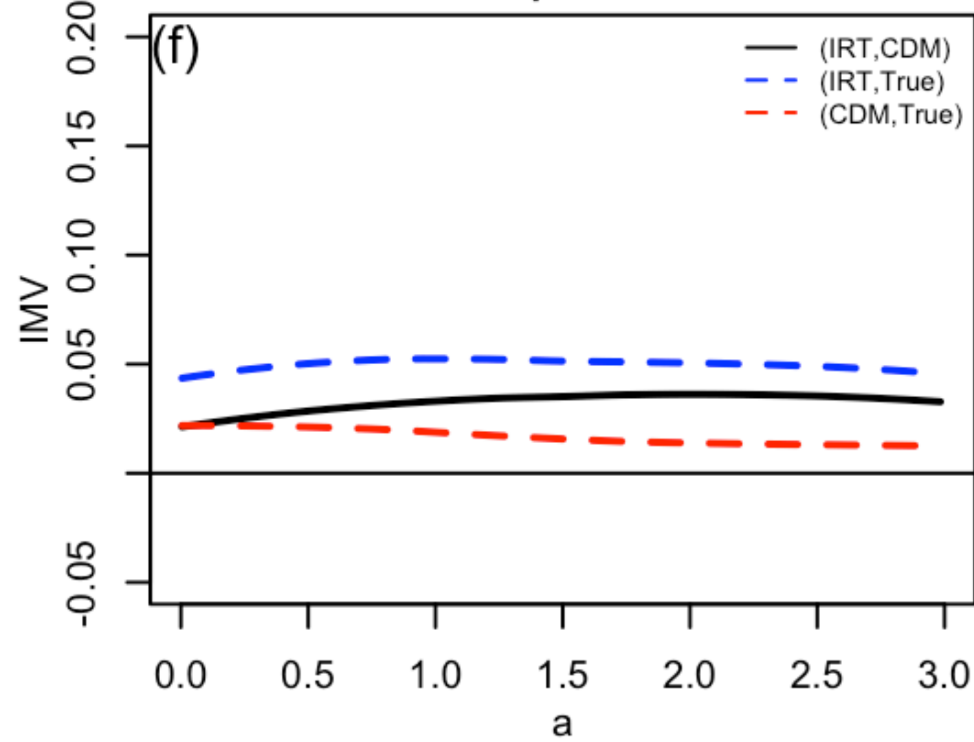
IMV ps = 0.6
