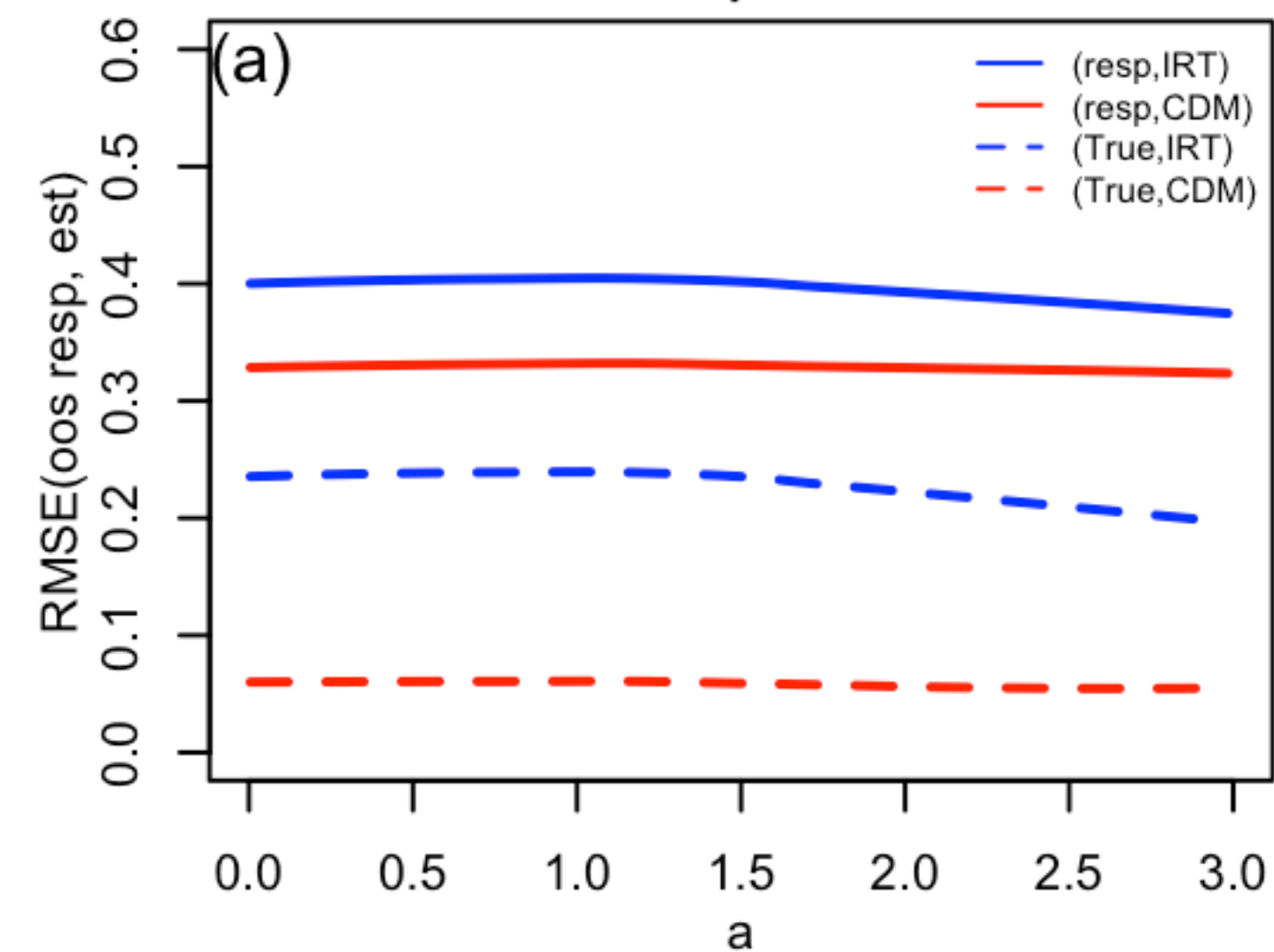
RMSE ps = 0.2
