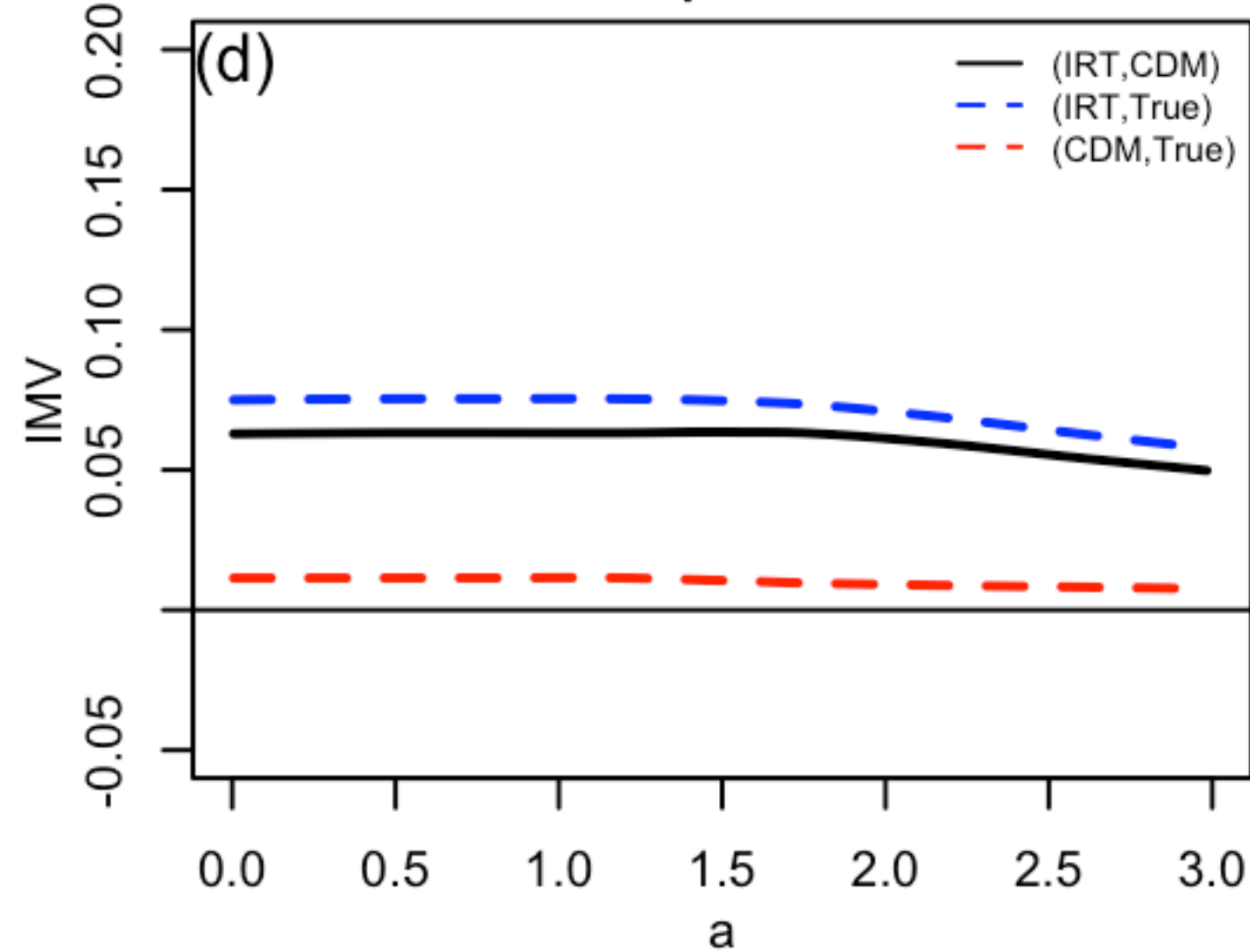
IMV ps = 0.4
