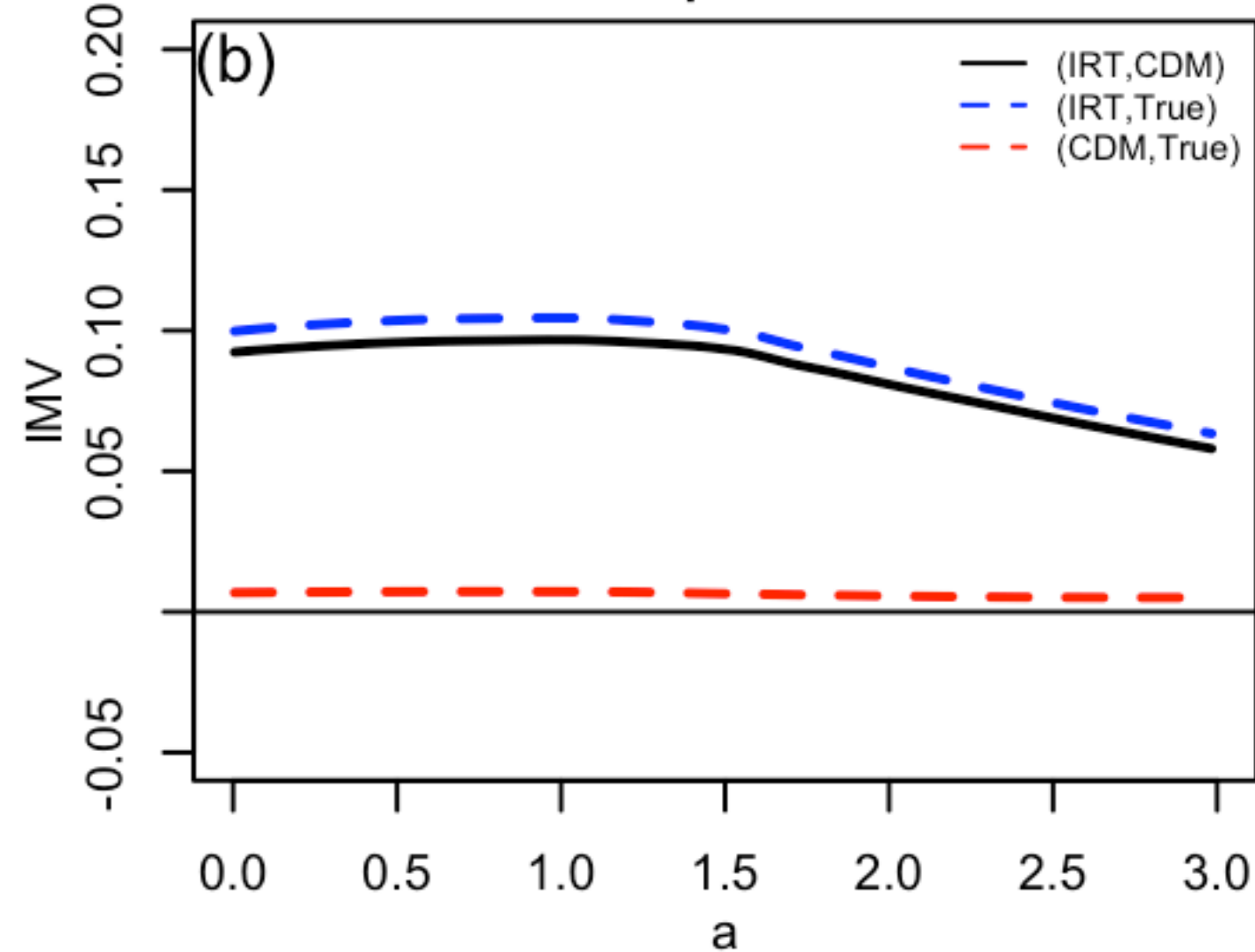
IMV ps = 0.2
