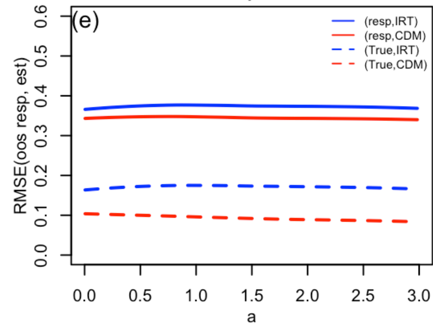
RMSE ps = 0.6
