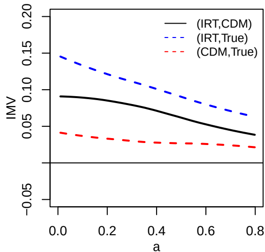
G-DINA with mp
