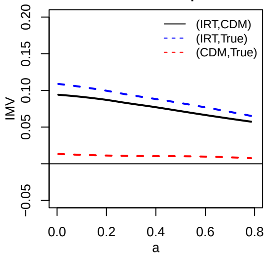
DINA with mp
