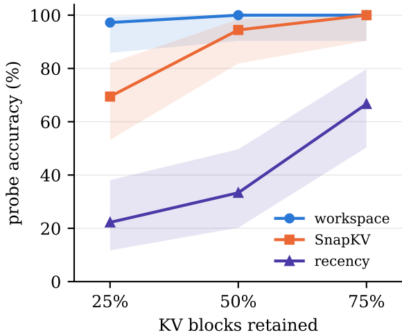
Qwen 2.5 7B
