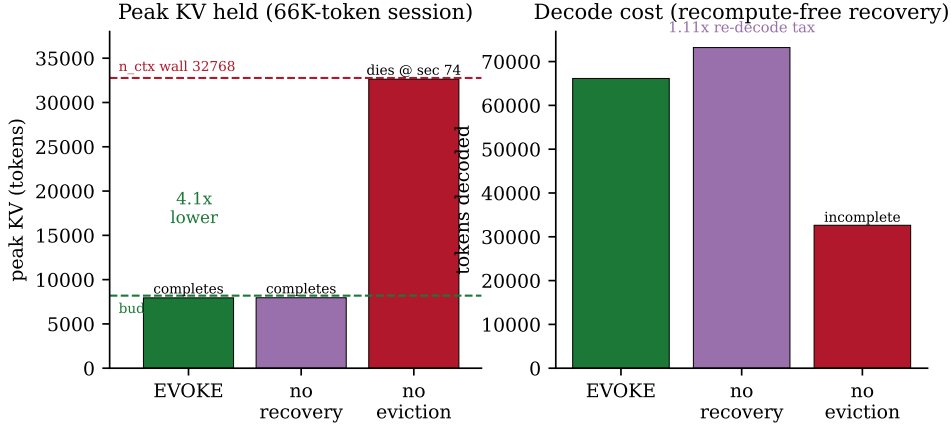
Figure 7: A 66K-token session under an 8K KV budget (Qwen 3-14B). Left: peak KV held; the no-eviction arm dies at the context wall mid-corpus. Right: tokens decoded; EVOKE recovers re-referenced sections without re-decoding them.
