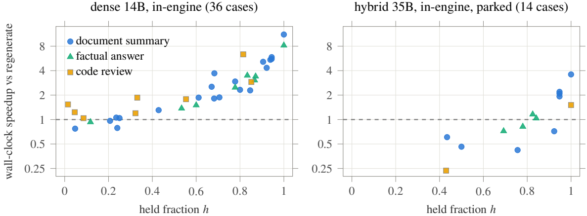
Figure 3: Speedup is governed by held fraction times answer length. Each point is one edit case (dashed line: parity). Left: on dense attention, holding pays almost everywhere above h \approx 0.2 . Right: on hybrid recurrent memory every divergence costs a suffix reprocess instead of a KV trim, so a win needs either zero divergences or length to amortize them; below parity sit short answers (13–41 tokens) and multi-divergence cases.
