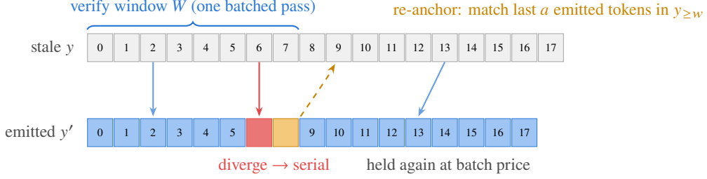
Figure 2: One divergence, resolved. Draft tokens from the stale answer are verified in windows. Position 6 is rejected: the model’s argmax is emitted, a short serial burst follows, and an a -gram match re-anchors the draft cursor past the changed span (skipping old token 8, which the edit invalidated). Everything downstream is held again.
