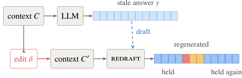
Figure 1: Reactive inference. An edit \delta turns context C into C' . Instead of regenerating the answer serially, REDRAFT replays the stale answer y as a self-speculative draft under C' : spans the model still agrees with are held at batched-verification price, the divergence is decoded serially, and drafting re-anchors so agreement after the edit’s blast radius is salvaged too.
