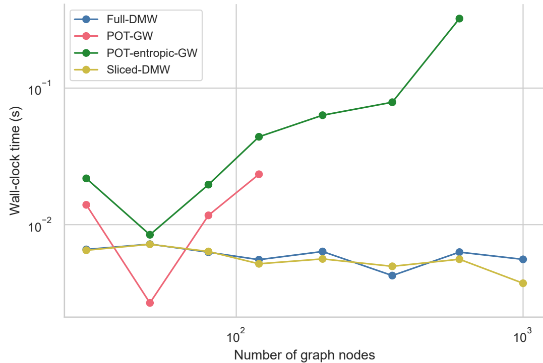
Scalability: DMW avoids node-level GW optimization
