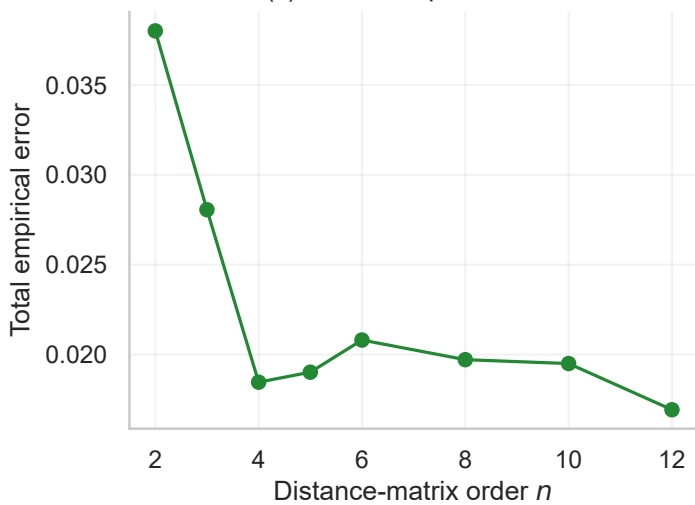
(c) Finite-sample tradeoff
