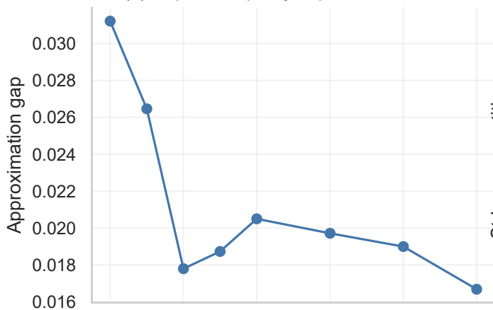
(a) Population proxy improves with order
