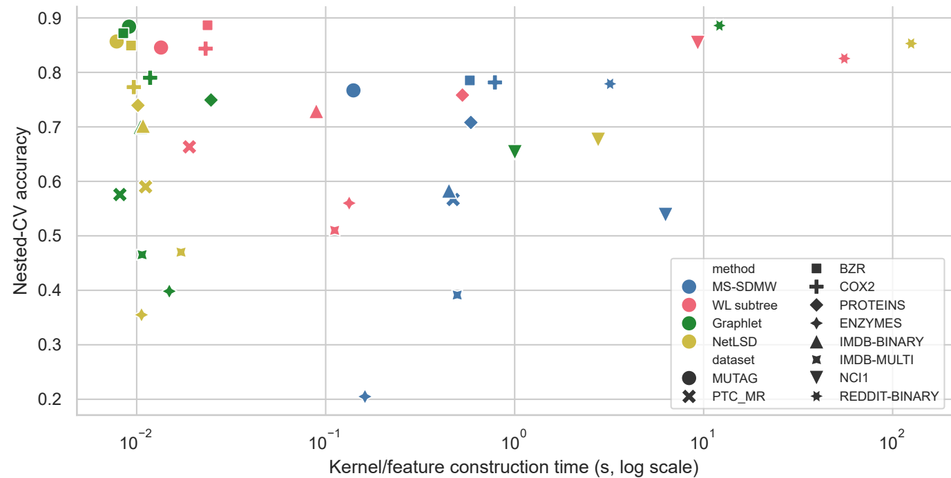
Accuracy--runtime profile on TU benchmarks
