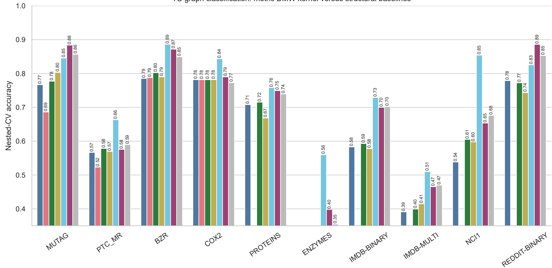
TU graph classification: metric DMW kernel versus structural baselines
