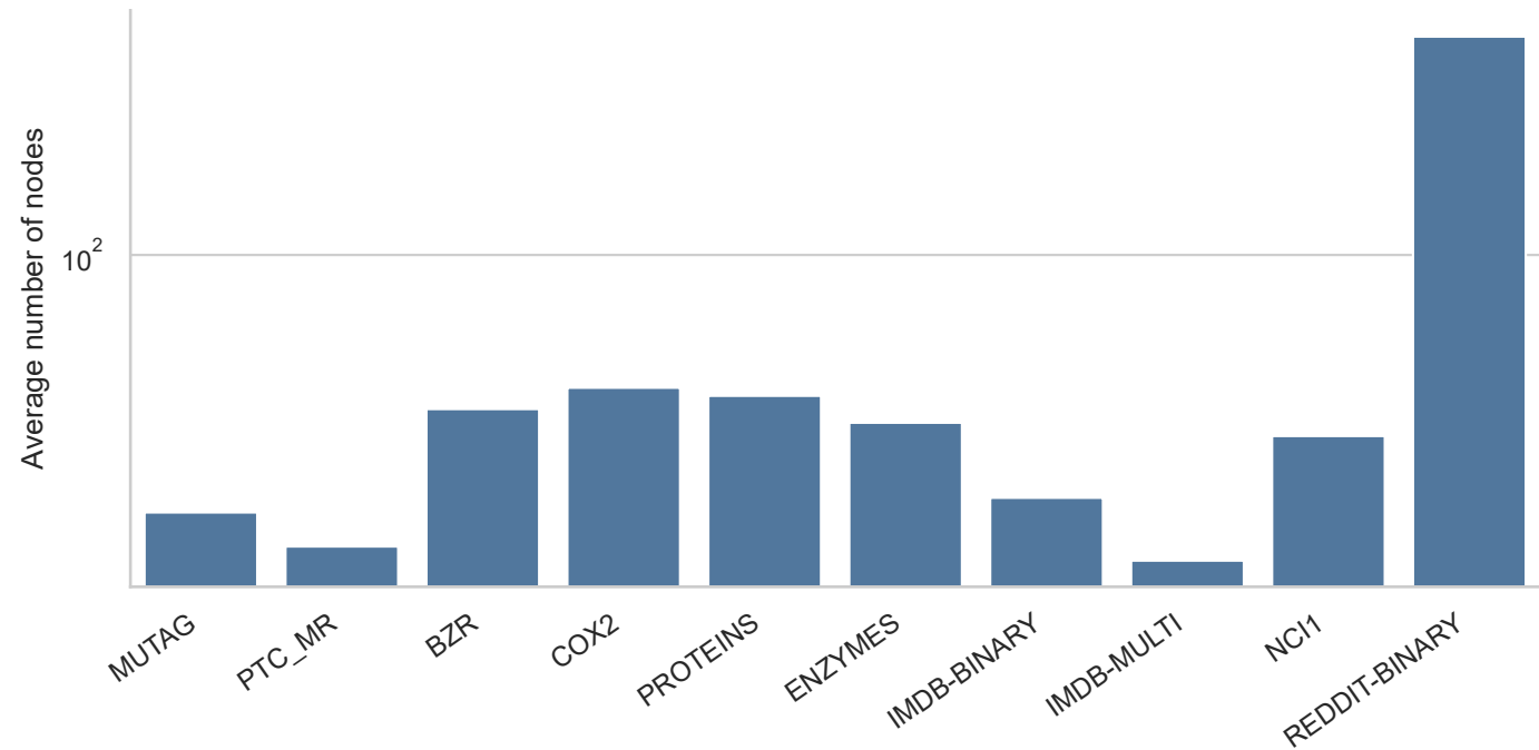
Scale of the TU benchmark suite
