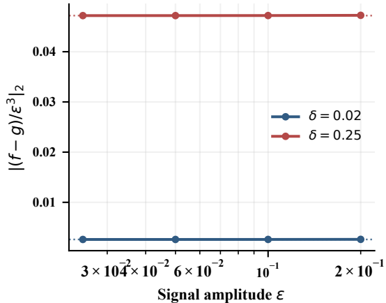
(b) Uncentered limit: \Delta_\delta[q]
