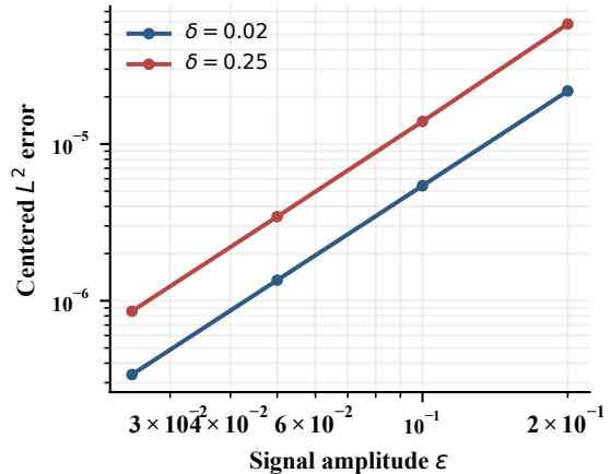
(c) Centered error: O(\varepsilon^2)
