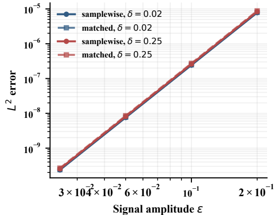
(a) Cubic truncation: O(\varepsilon^5)
