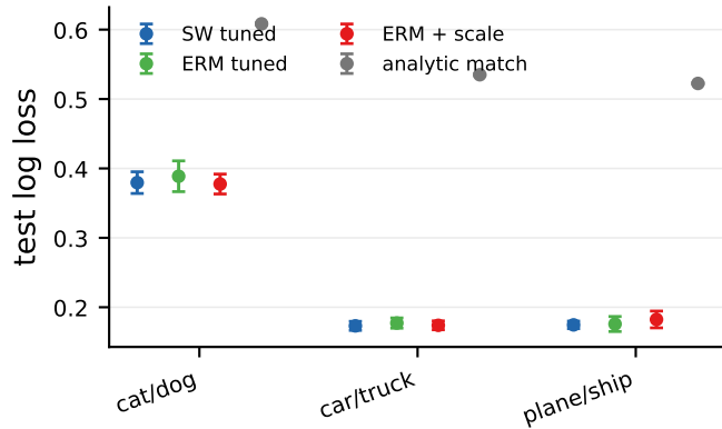
ResNet-18
