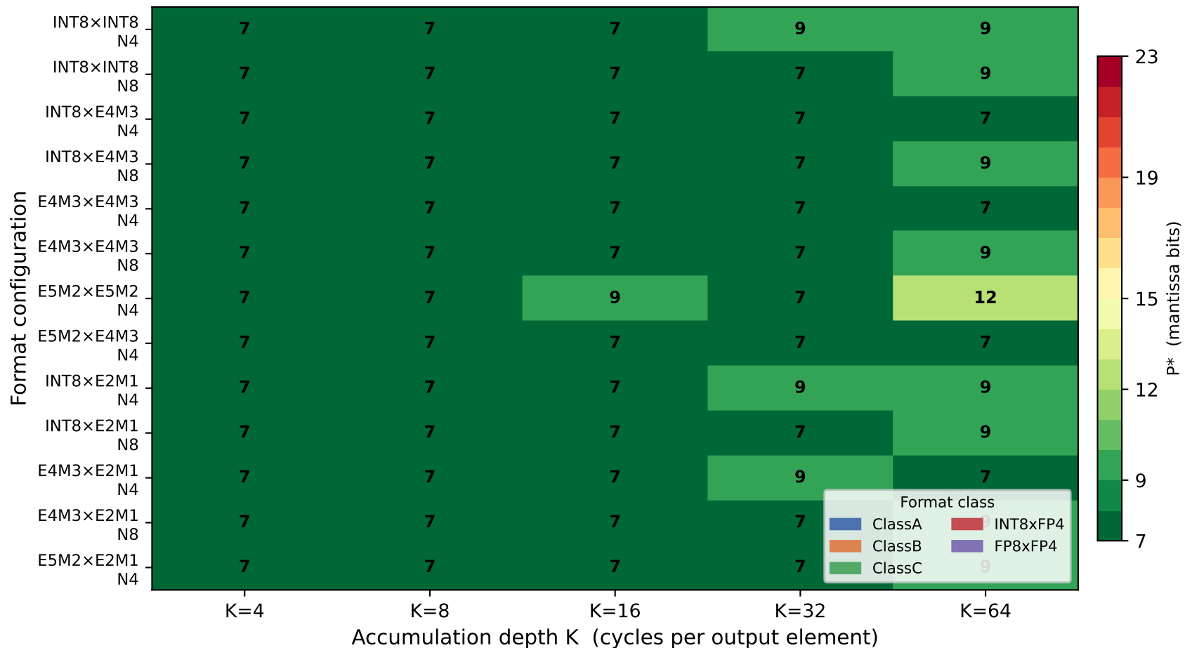
Fig 1 — Minimum sufficient accumulator mantissa bits P^* (normErr criterion: full-pipeline error \leq 110\% of FP32 baseline)
