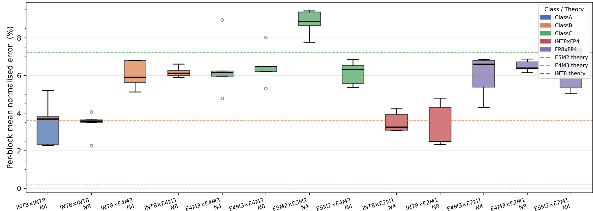
Fig 2 — Requant noise floor distribution across K values (accMantBits=23 / FP32 accumulator; pure requantisation noise)
