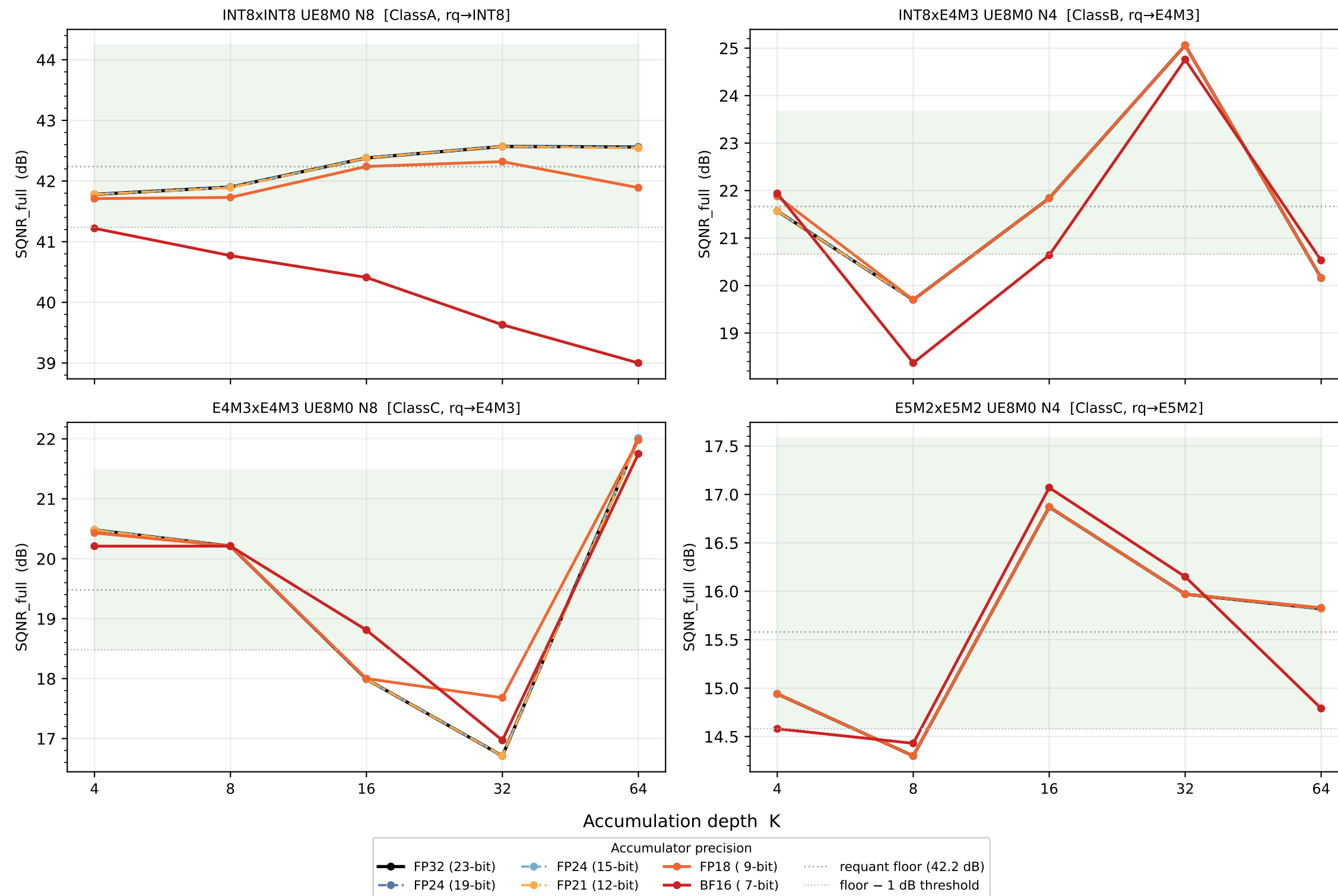
Fig 4 — Full-pipeline SQNR vs K at different accumulator precisions (green band = within 1 dB of requant noise floor → lossless)
