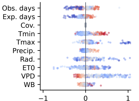
Permutation-SHAP contribution
