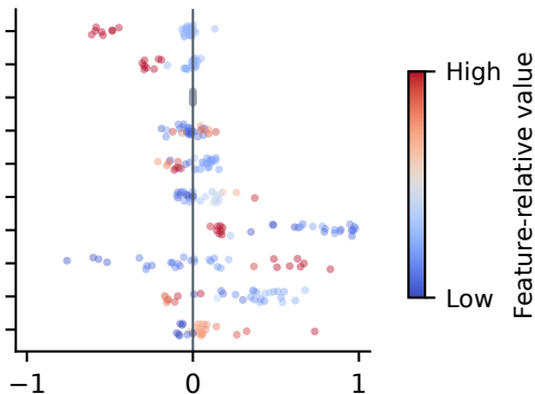
Permutation-SHAP contribution
