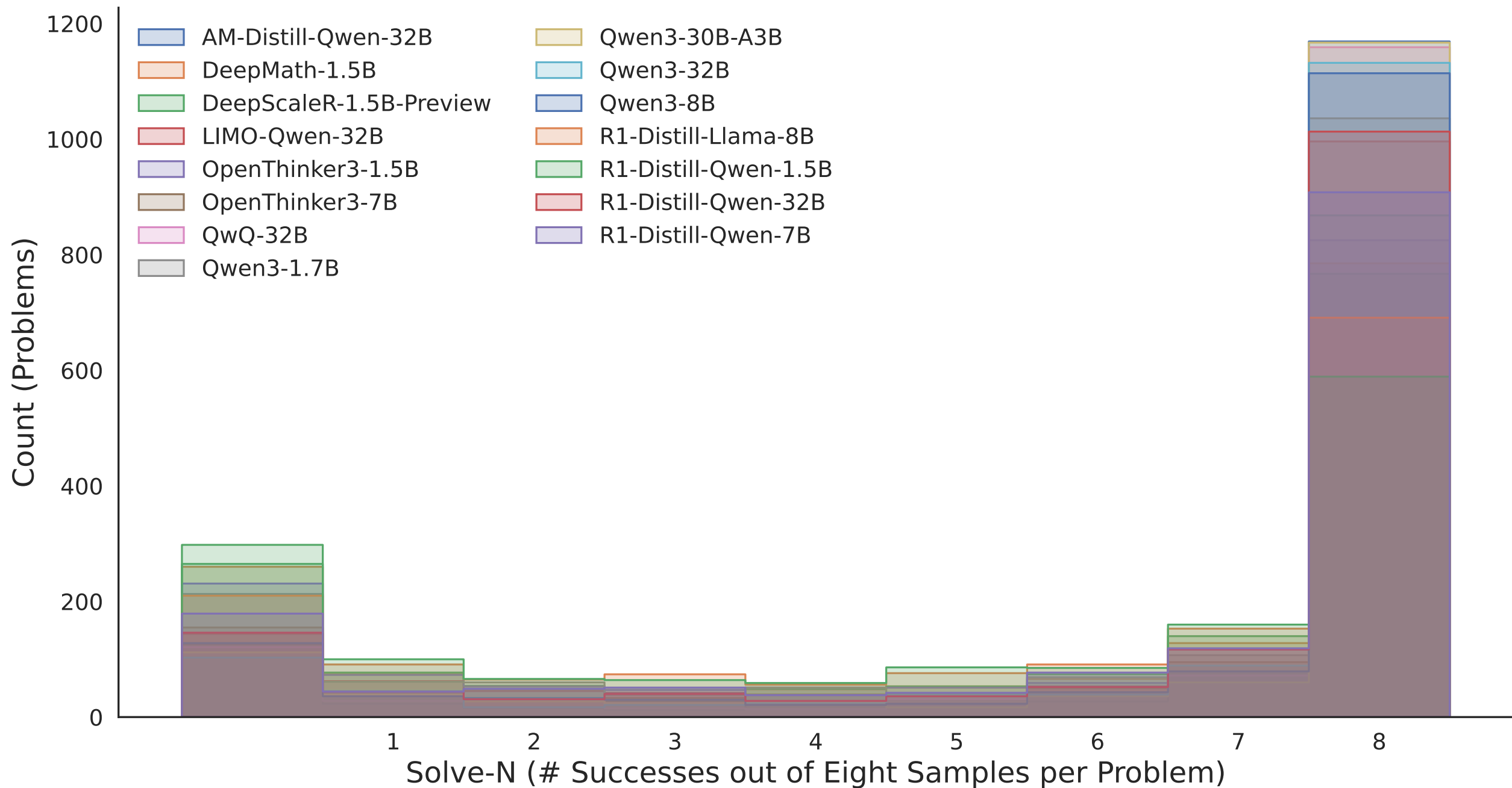
Distribution of Solve-N Across Benchmarks and LLMs
