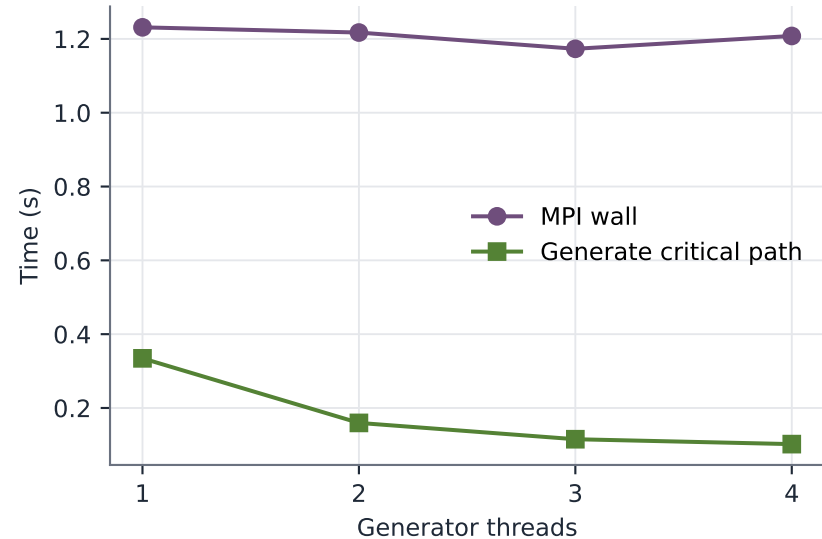
Advanced: generator-thread tuning
