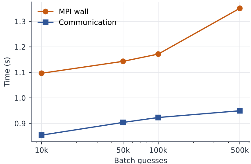
Advanced: batch-size tuning
