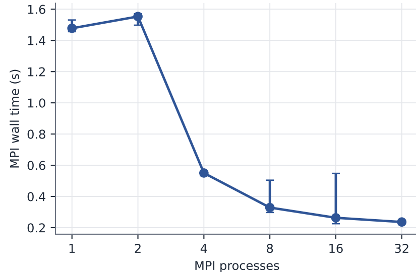
Base: parallel-stage wall time
