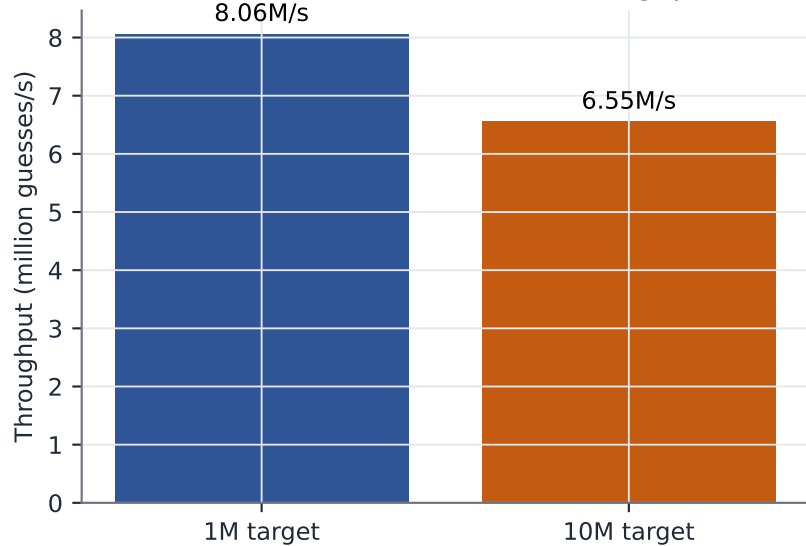
Advanced NP=4: effective throughput
