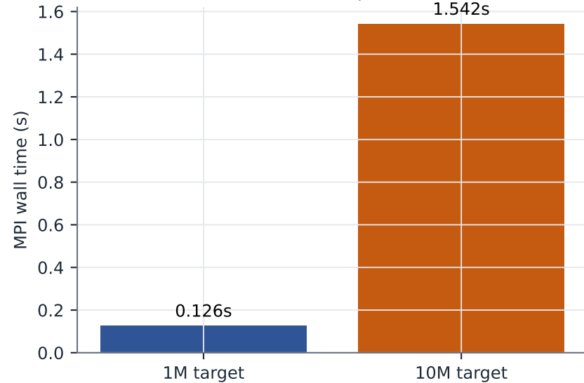
Advanced NP=4: problem size
