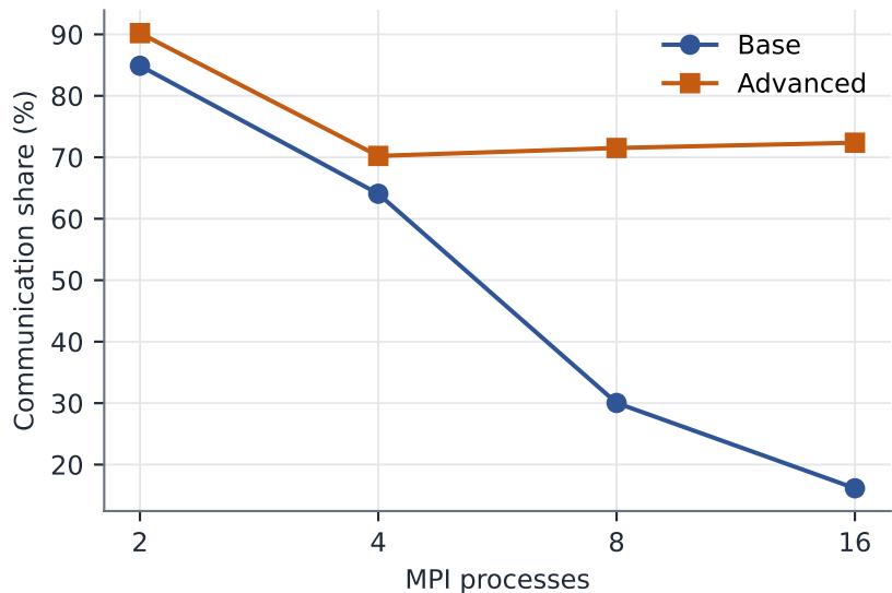
Communication in MPI wall time
