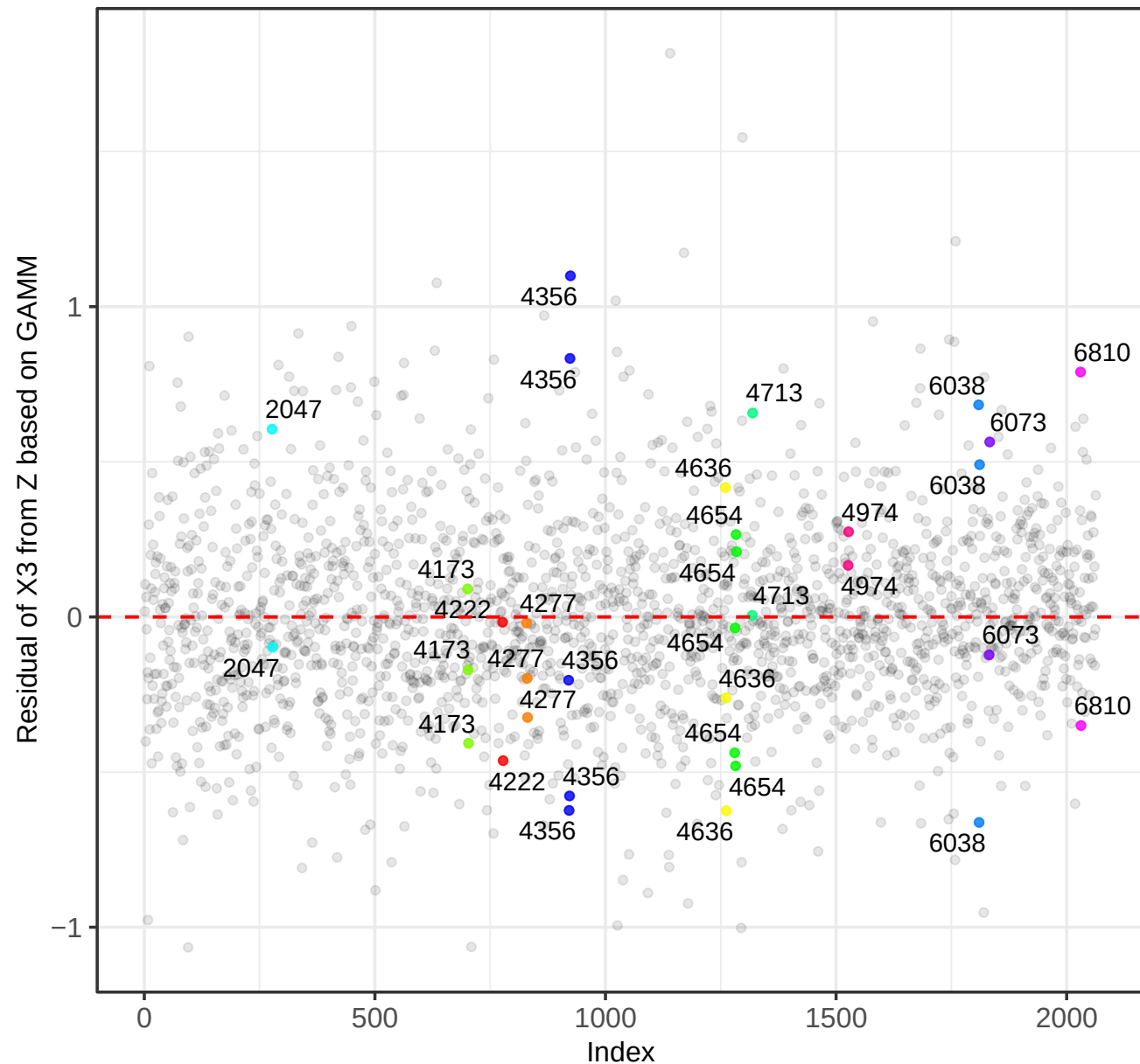
Residuals Plot for X3 utilizing the EGCM
