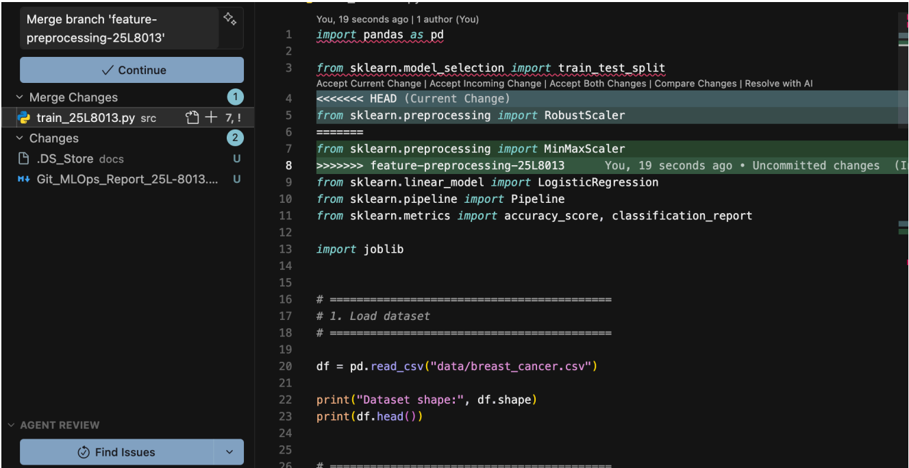
Screenshot 3 (required) — VS Code merge conflict interface showing conflict markers
