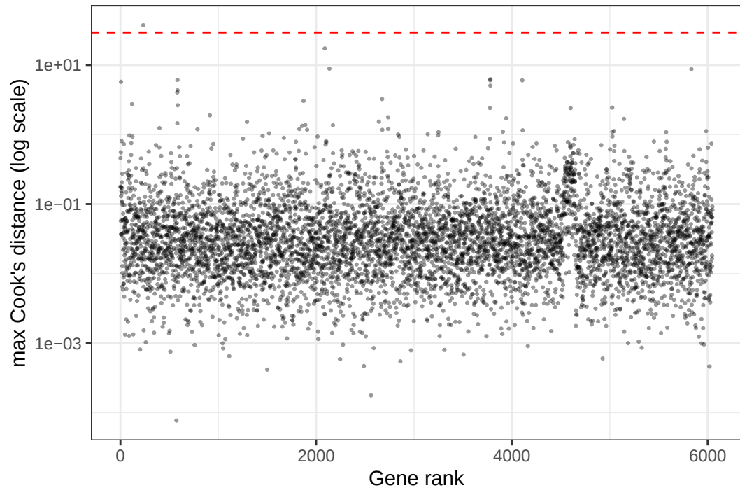
Cook's distance (cutoff 29.46; 1 genes above)
