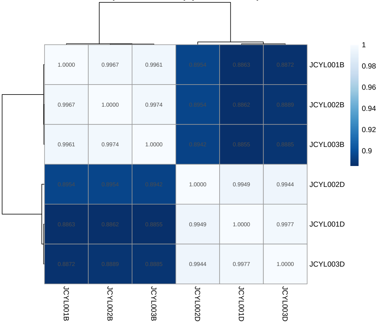
Sample correlation (Spearman, VST)
