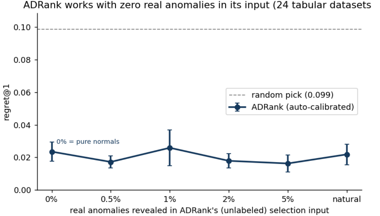
Figure 5. Regret@1 versus the fraction of real anomalies present in ADRank's unlabeled selection input, mean over 24 tabular datasets and three seeds (error bars are the standard error over datasets). The curve is flat: regret at 0% real anomalies (pure normals, 0.024) is indistinguishable from regret at the natural contamination rate (0.022), and every level sits 4-6 \times below the random-pick baseline (0.099).
