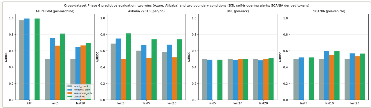
Figure 4. Held-out predictive AUROC by feature set across the four temporally-split traces (Azure, Alibaba, BGL, SCANIA). The combined feature set leads on Azure and Alibaba; BGL and SCANIA sit at the no-signal boundary.
