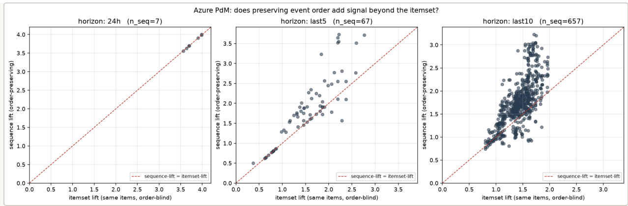
Figure 3. Itemset lift versus sequence lift for Azure patterns. Points above the diagonal are patterns whose ordered form carries more failure signal than their unordered co-occurrence, the effect the count-preserving null of §4.7 isolates.
