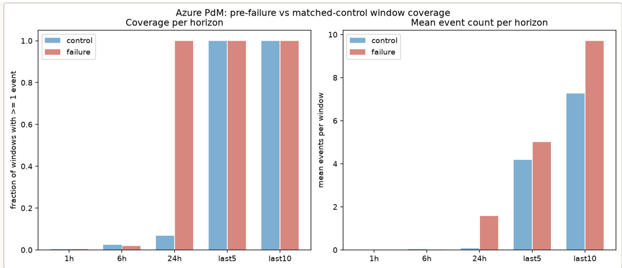
Figure 1. Event coverage of Azure pre-failure windows by horizon: the mean number of events per window grows with horizon length, which sets how much order information each horizon can carry.
