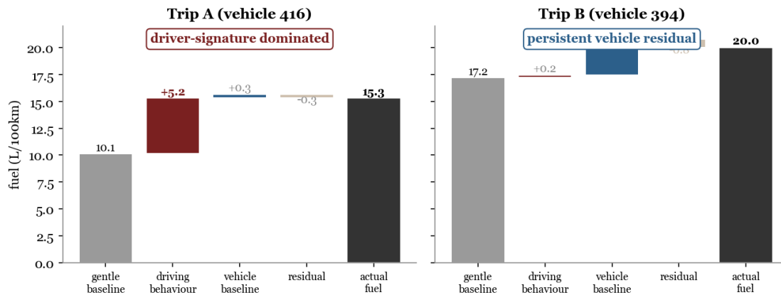
Figure 9. Two real trips, same elevated fuel, opposite cause. The decomposition separates a driver-dominated trip (A) from a vehicle-dominated trip (B).
