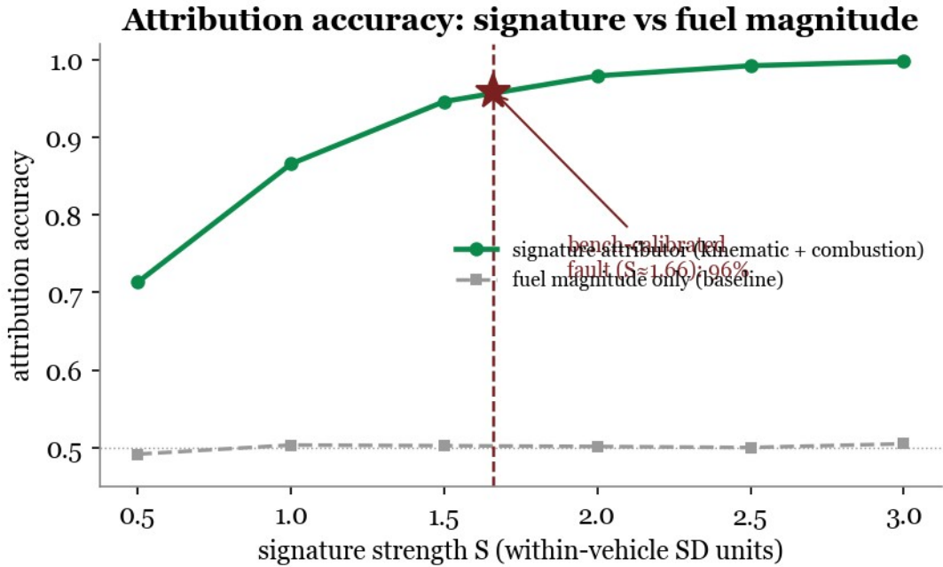
Figure 7. Attribution accuracy versus signature strength, reaching 95.9% at the bench-calibrated fault magnitude while the fuel-magnitude baseline stays at chance. This classifier is trained on the injected labels and is therefore an upper bound; Section 8.4 reports the transfer result that does not use them.
