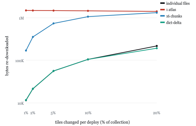
Figure 4. Warm-cache re-download: bytes a returning client fetches after a deploy changes a fraction of a 200-tile WebP collection (log scale; full fresh download 1,474,036 B; mean of 20 random deploys per rate). A single atlas re-fetches almost everything on any change; 16 chunks scale with churn; dictionary-delta serving tracks the individual-file optimum and undercuts it at high churn.
