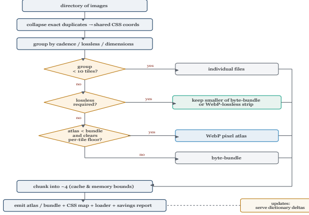
Figure 5. The construction heuristic as implemented in atlas_optimizer . Exact duplicates collapse to shared coordinates; tiles are grouped by update cadence, lossless requirement, and dimensions; each group is routed by a short decision cascade to individual files, a pixel atlas, or a byte-bundle. The lossy branch is decided by measurement: a pixel atlas is chosen only if it is smaller than the byte-bundle and clears a per-tile SSIM floor, and lossless groups keep the smaller of a byte-bundle and a WebP-lossless strip. Groups are chunked for bounded cache invalidation and memory, and the tool emits the atlas and bundle files, a CSS coordinate map, a loader, and a savings report; piecewise updates can be served as dictionary deltas. This is the procedure evaluated against the oracle in Table 9.
