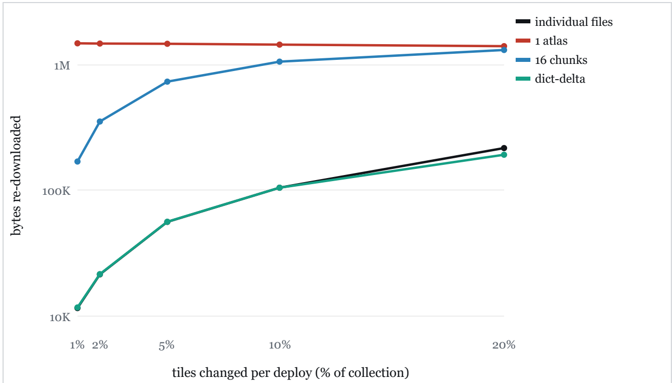
Figure 5. Warm-cache re-download: bytes a returning client fetches after a deploy changes a fraction of a 200-tile WebP collection (log scale; full fresh download 1,474,036 B; mean of 20 random deploys per rate). A single atlas re-fetches almost everything on any change; 16 chunks scale with churn; dictionary-delta serving tracks the individual-file optimum and undercuts it at high churn.
