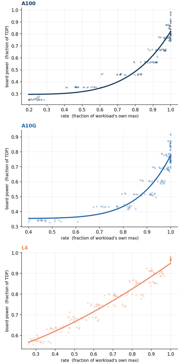
Figure 2. The response law P(\theta) = P_0 + a\theta^\beta is a card property. One panel per GPU (A100, A10G, L4); each dot is a measured operating point for one of the 20 workloads in the loaded regime, with the rate normalized to that workload's own maximum and power to the card's TDP. All workloads closely follow a single fitted law per card (line), showing the exponent travels with the card, not the model: pooled fit R^2 of 0.92 (A100), 0.88 (A10G), and 0.95 (L4), with \beta from about 1.5 on the L4 to 7.4 on the A10G.
