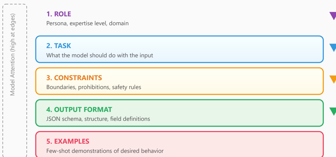
Figure 11.1.6: A production system prompt follows a layered architecture. Models attend most strongly to early and late content.
