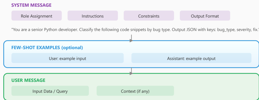
Figure 11.1.2: The structural components of a prompt mapped to chat API message roles.
