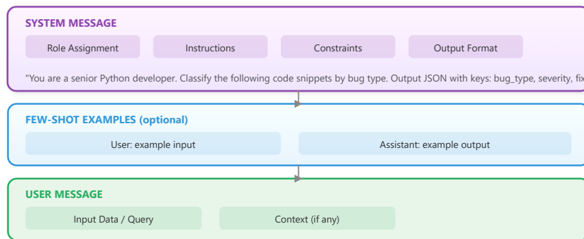
Figure 11.1.2: The structural components of a prompt mapped to chat API message roles.
