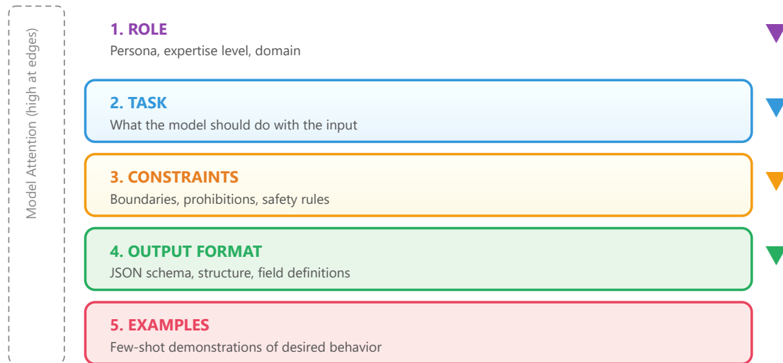
Figure 12.1.3a: A production system prompt follows a layered architecture. Models attend most strongly to early and late content.
