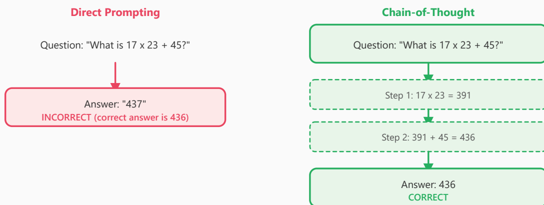
Figure 11.2.3: Direct prompting compresses all reasoning into one step; CoT decomposes it into verifiable intermediate steps.
