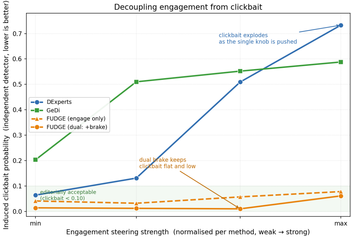
Figure 6. Decoupling engagement from clickbait. Induced clickbait (independent detector) as each method is steered from weak to strong engagement, with the steering strength normalised per method. The single-axis baselines DExperts and GeDi cannot raise engagement without raising clickbait: their induced clickbait climbs steeply with steering (DExperts to 0.73, GeDi to 0.59). The dual guide’s clickbait brake holds induced clickbait low and flat across the range (below 0.06); the engage-only FUDGE curve (dashed) shows that the multiplicative guidance is already low-clickbait and the brake lowers it further. This decoupling, which the single-axis baselines cannot express, is the dual-control contribution.
