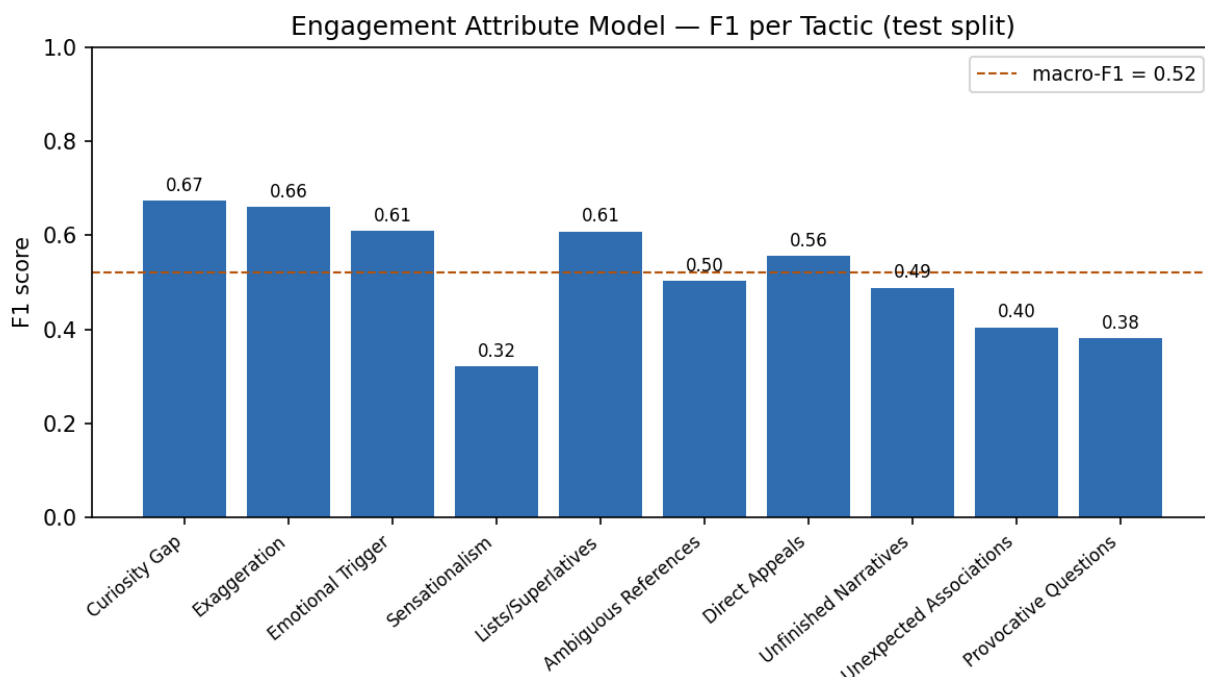
Figure 3. Per-tactic F1 of the engagement attribute model on single-tactic test examples (macro-F1 = 0.52).
