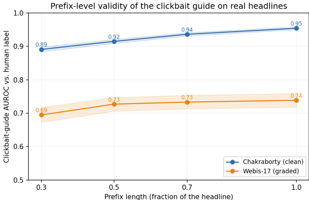
Figure 7. Prefix-level validity of the clickbait guide. AUROC of the guide’s prefix score against the parent headline’s human label as the prefix grows from 30% to 100% of the headline, on the Chakraborty and Webis corpora (shaded 95% CI). The guide provides a valid, monotonically strengthening signal from an early prefix.
