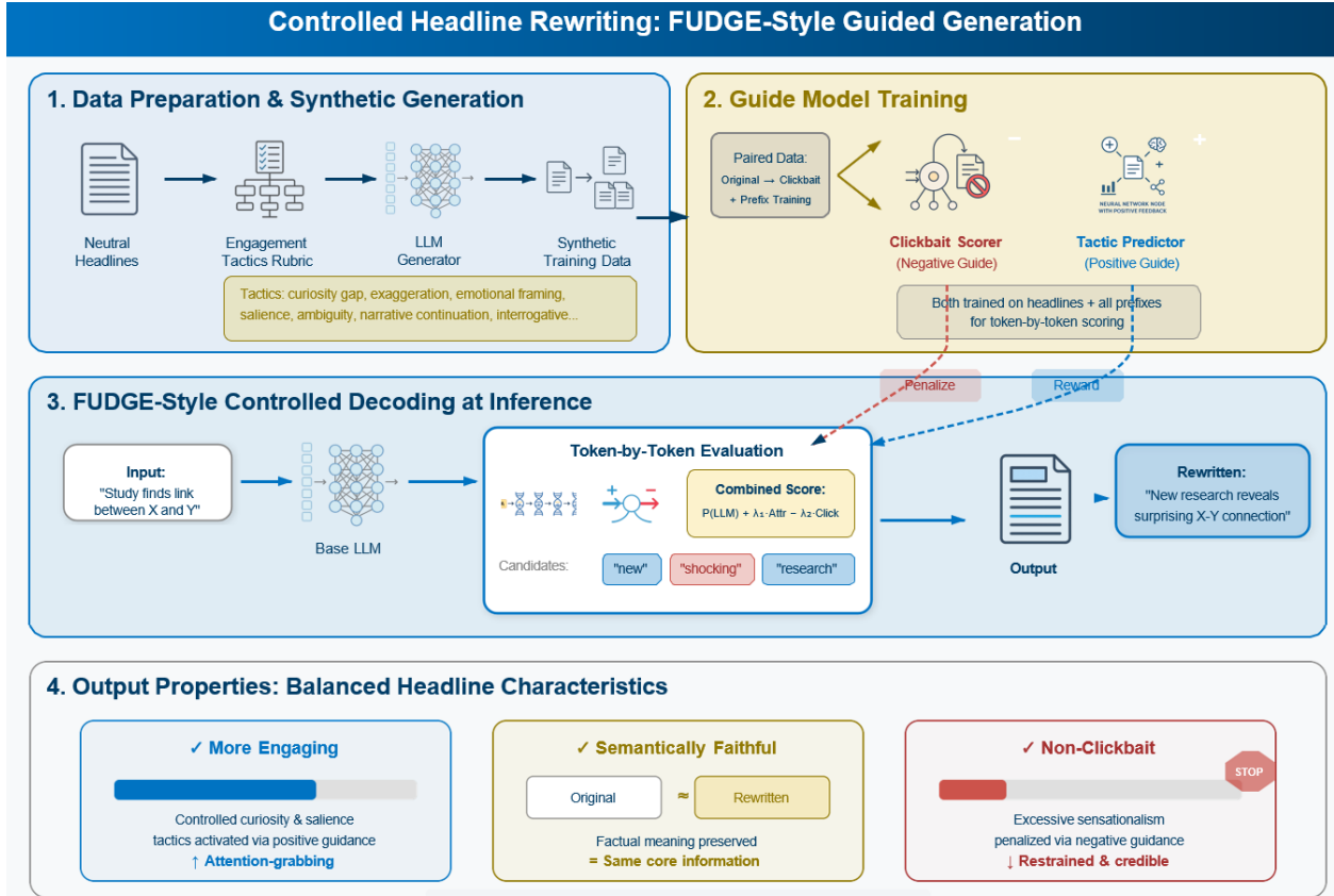
Figure 1. General flow of the proposed rubric-based and FUDGE-guided headline rewriting approach.
