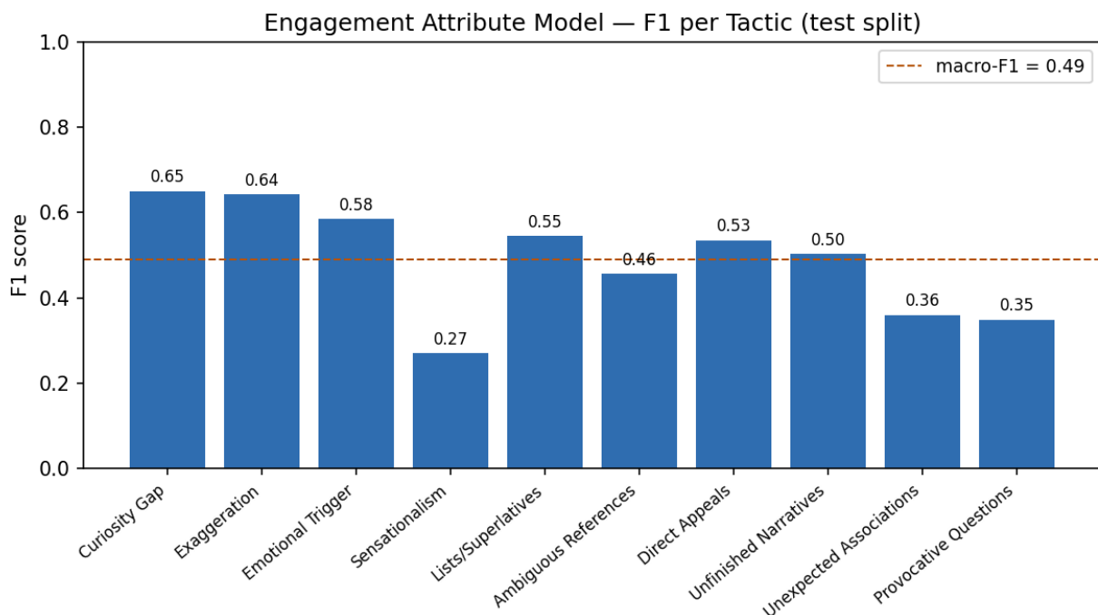
Figure 3. Per-tactic F1 of the engagement attribute model on single-tactic test examples (macro-F1 = 0.49).
